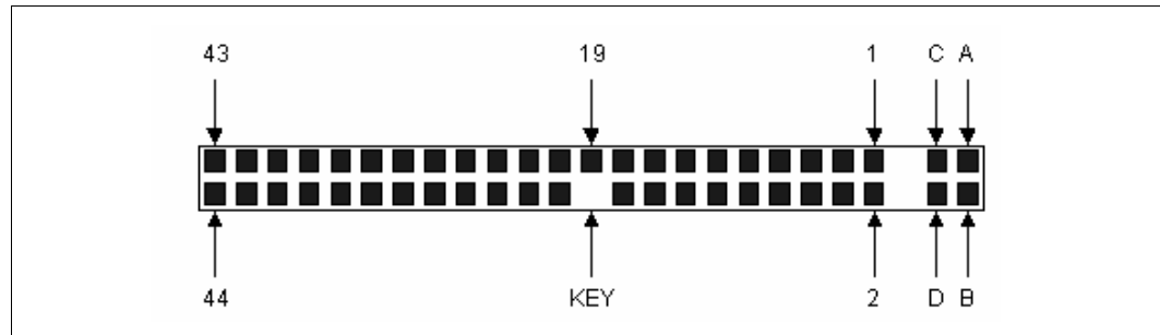
Figure 2-2. Pin Locations
