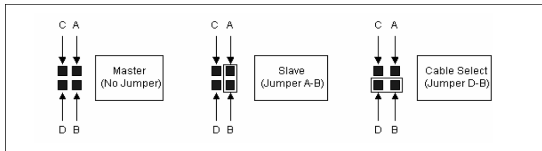
Figure 2-3. Jumper Settings
